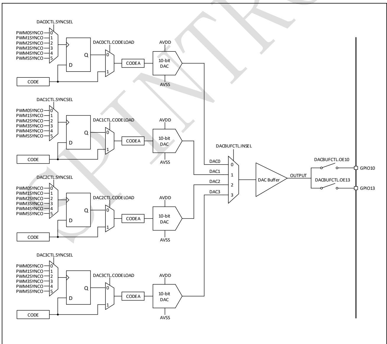
Figure 16-1: Buffered DAC block diagram
