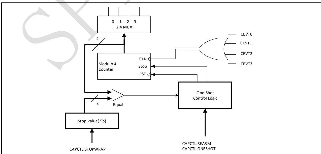
Figure 11-6: Details of the continuous/one-shot block
