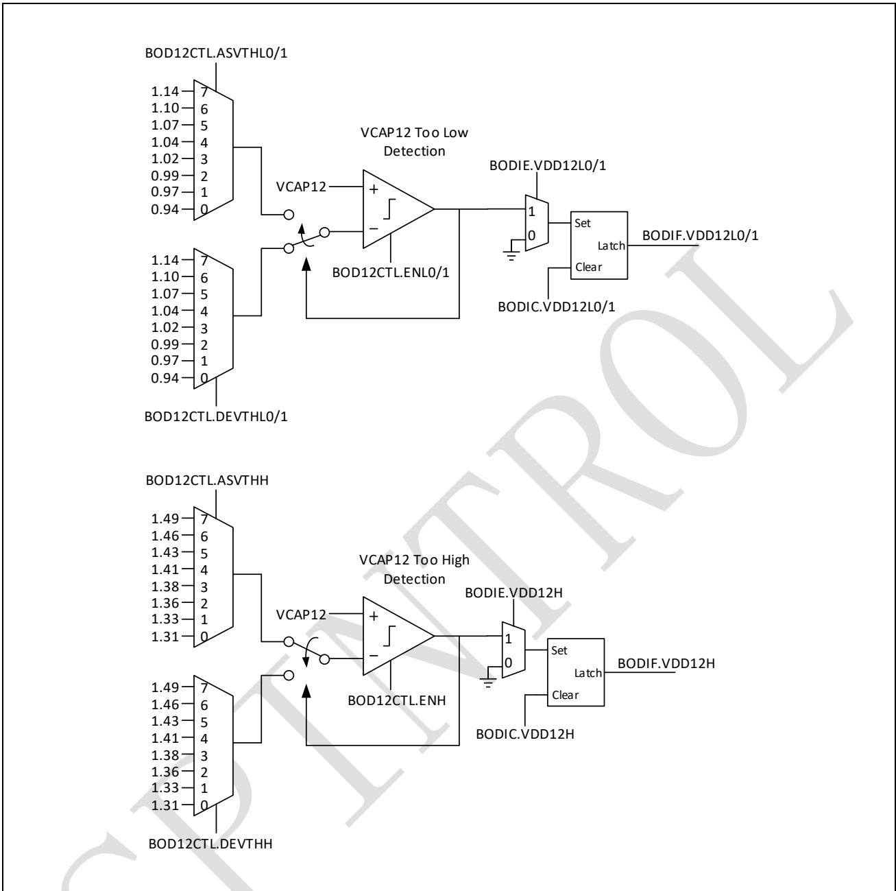
Figure 2-3: 1.2V domain brown-out detector diagram
