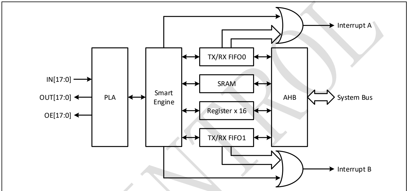
Figure 21-1: SIO architecture diagram
