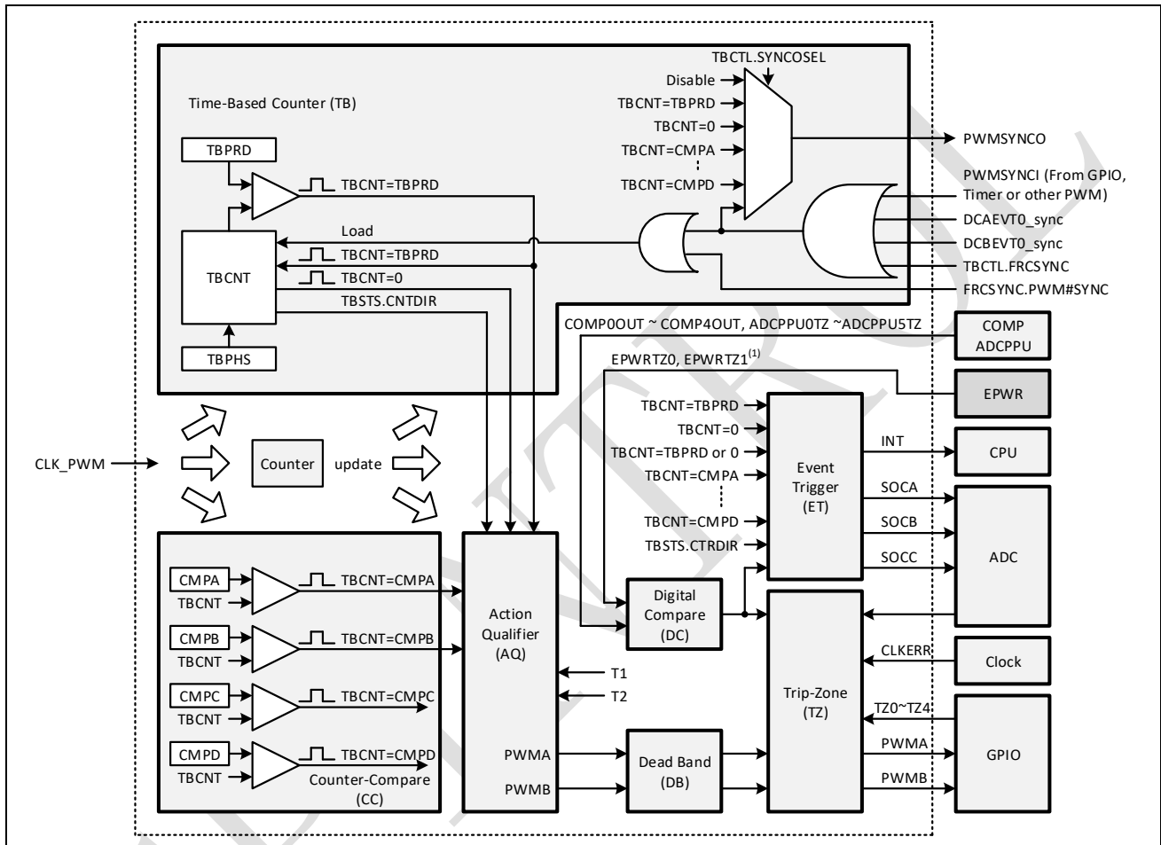
Figure 10-2: PWM architecture
