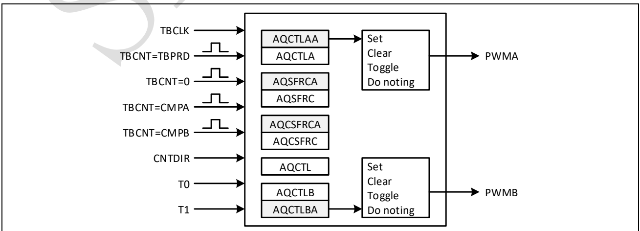
Figure 10-8: Action-Qualifier sub-module inputs and outputs
