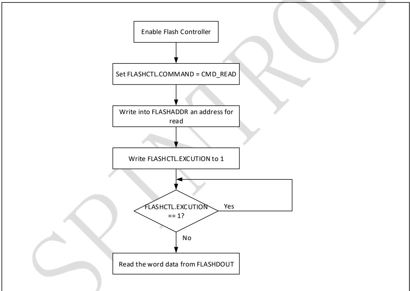
Figure 20-3: Flash memory reading procedure
