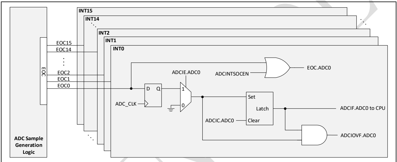
Figure 12-10: Interrupt structure
