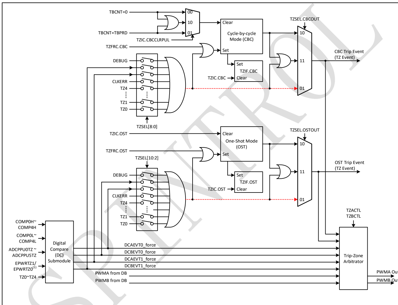
Figure 10-14: Trip-Zone sub-module logic
