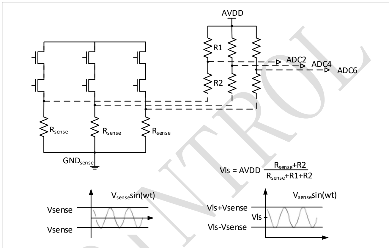
Figure 14-3: Single-ended sensing of driver FET currents
