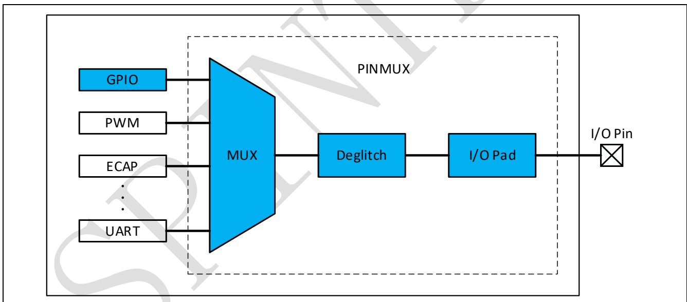
Figure 4-1: Structure diagram of I/O control
