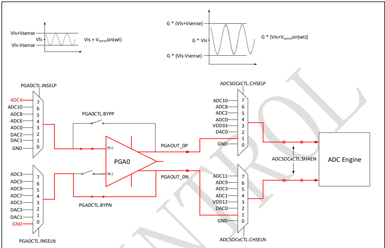
Figure 14-4: PGA0 sample ADC4 in single-ended mode
