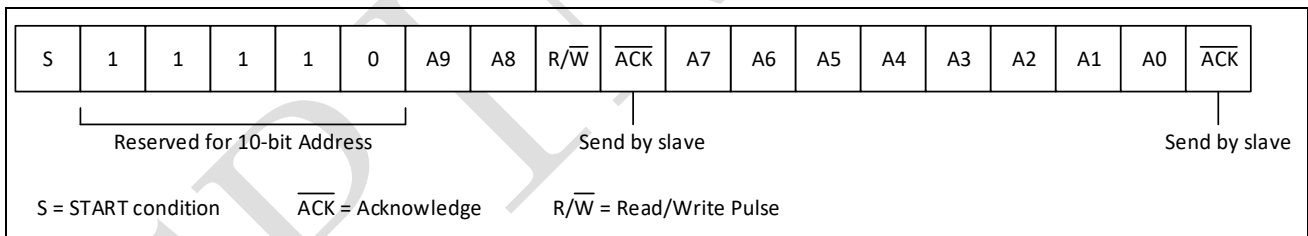
Figure 18-4: 10-bit address format
