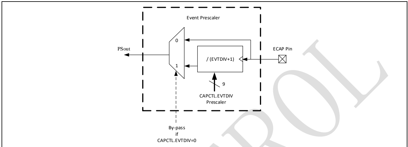
Figure 11-4: Event prescaler control
