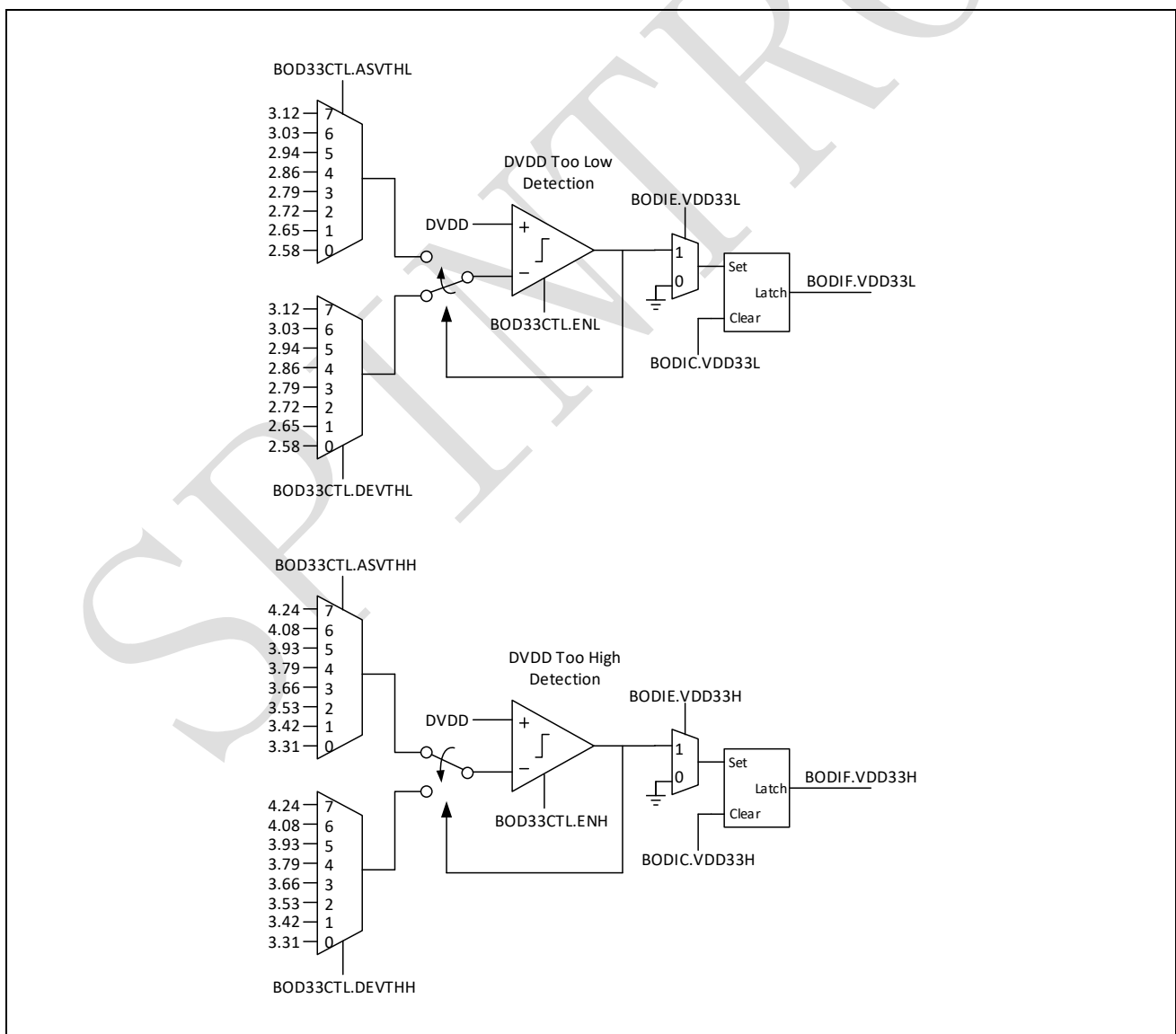
Figure 2-2: 3.3V domain brown-out detector diagram
