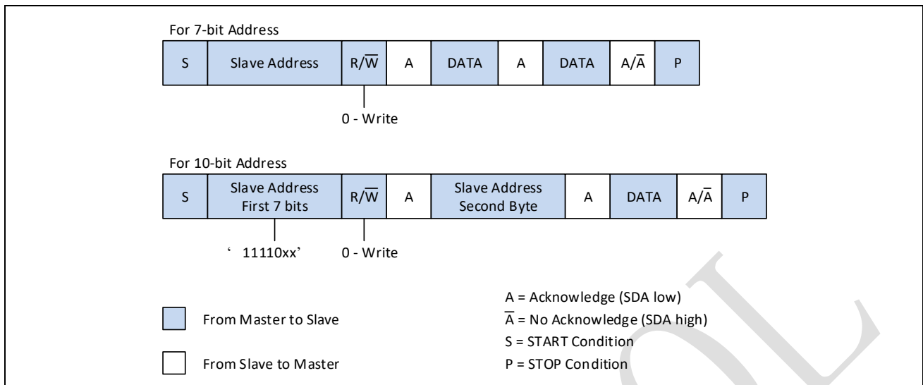
Figure 18-5: Master-transmitter protocol
