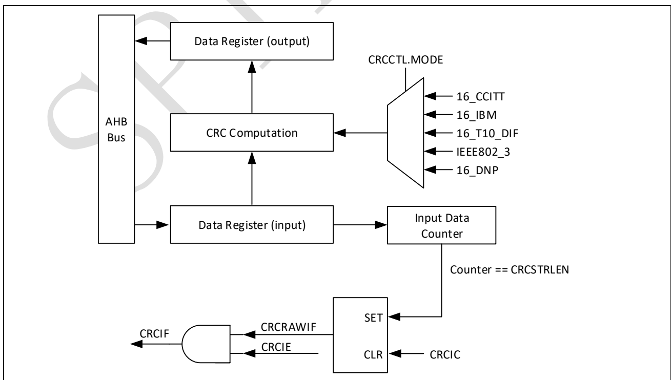
Figure 7-1: CRC block diagram
