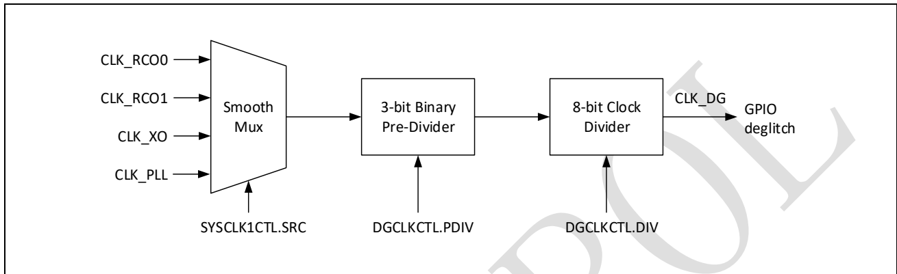
Figure 3-10: GPIO deglitch clock diagram
