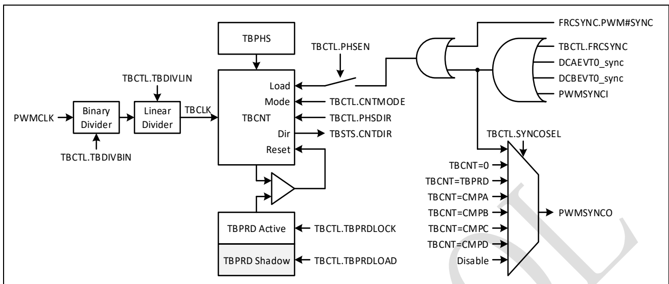
Figure 10-3: Time-Base sub-module signals
