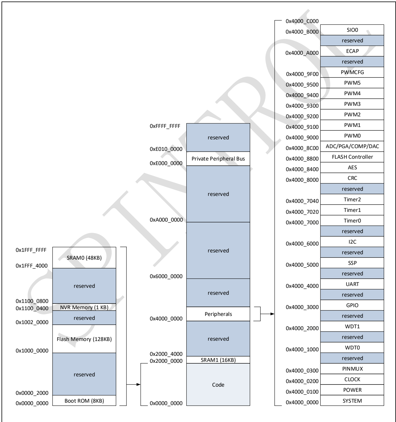
Figure 1-3: SPC1168 memory map
