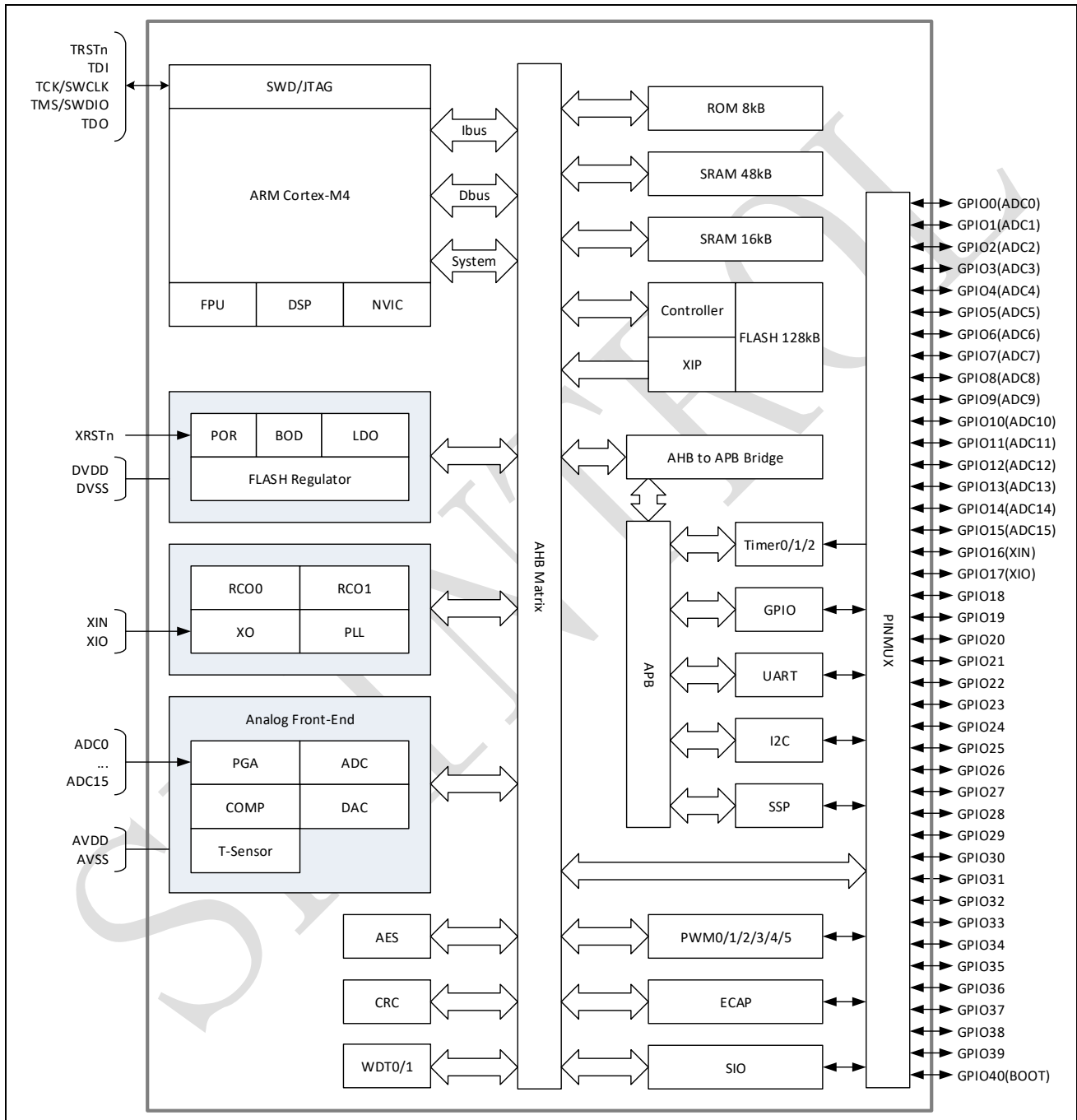
Figure 1-1: Block diagram of SPC1168
