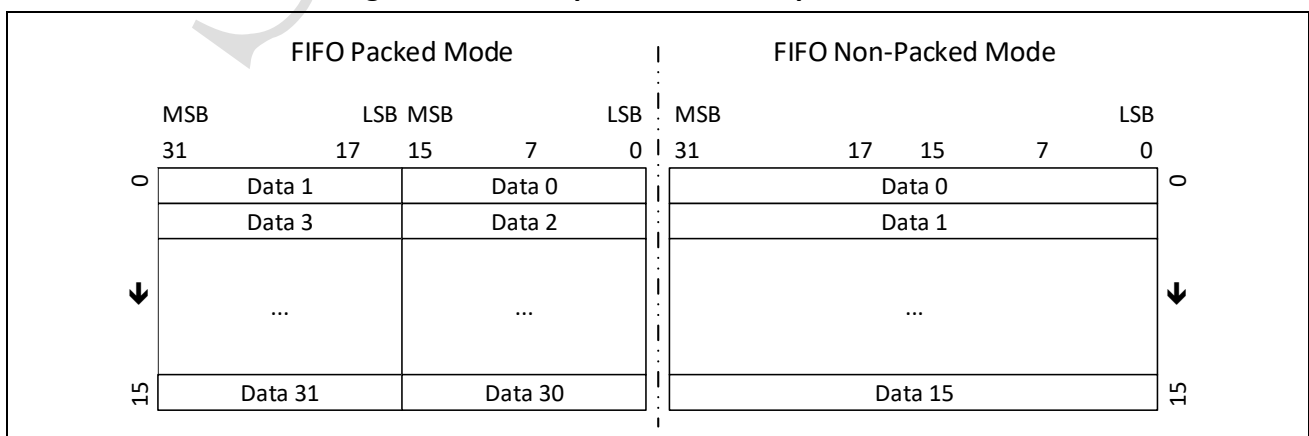
Figure 19-3: FIFO packed and non-packed mode
