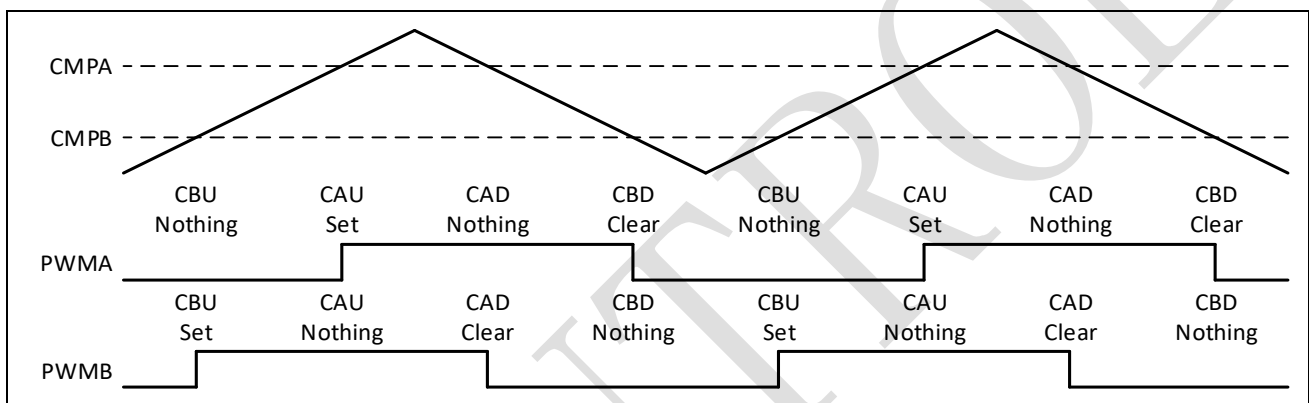
Figure 10-10: Up-Down-Count, dual edge asymmetric waveform of Action-Qualifier
