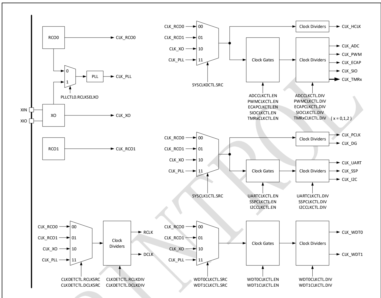
Figure 1-2: SPC1168 clock tree
