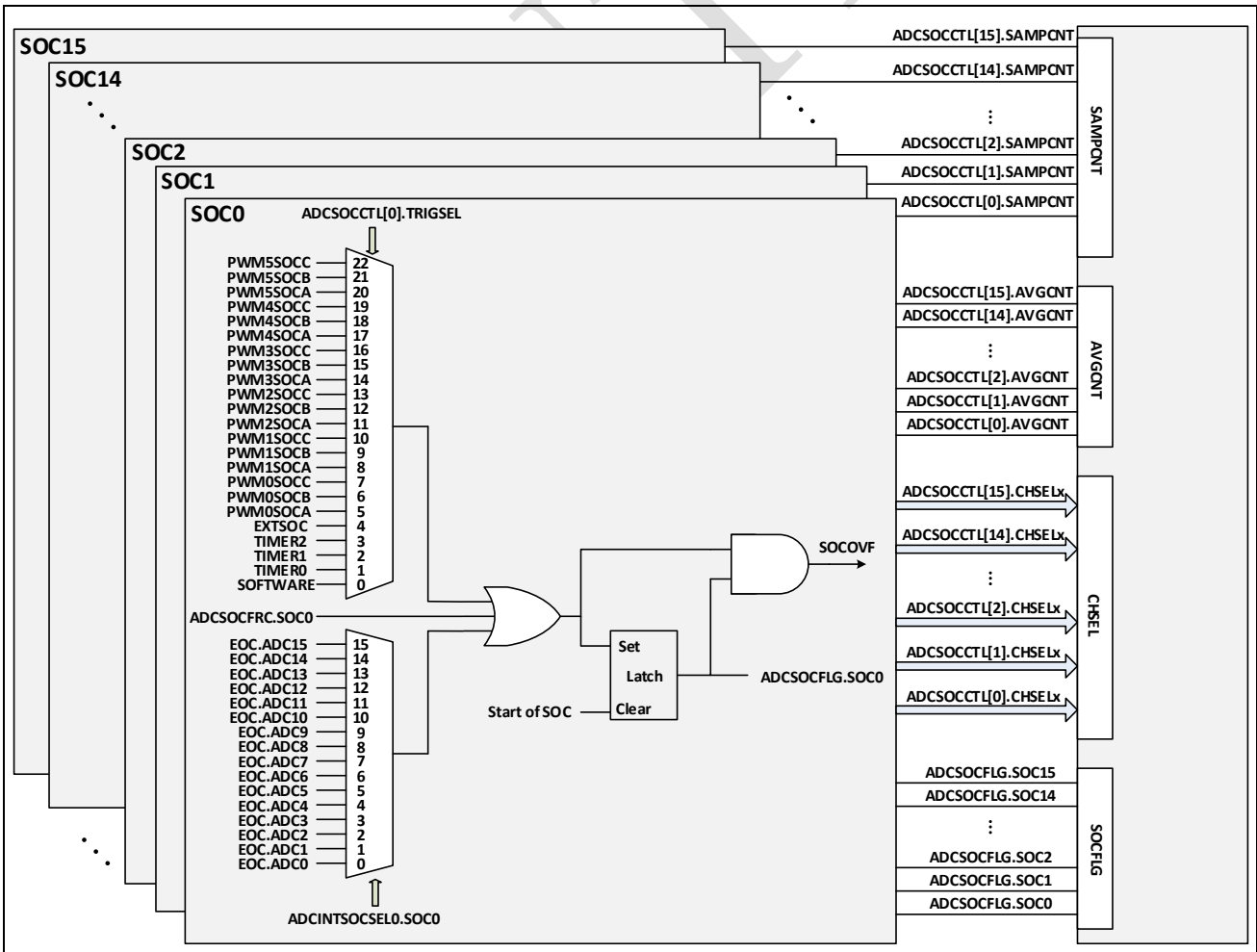
Figure 12-2: SOC block diagram
