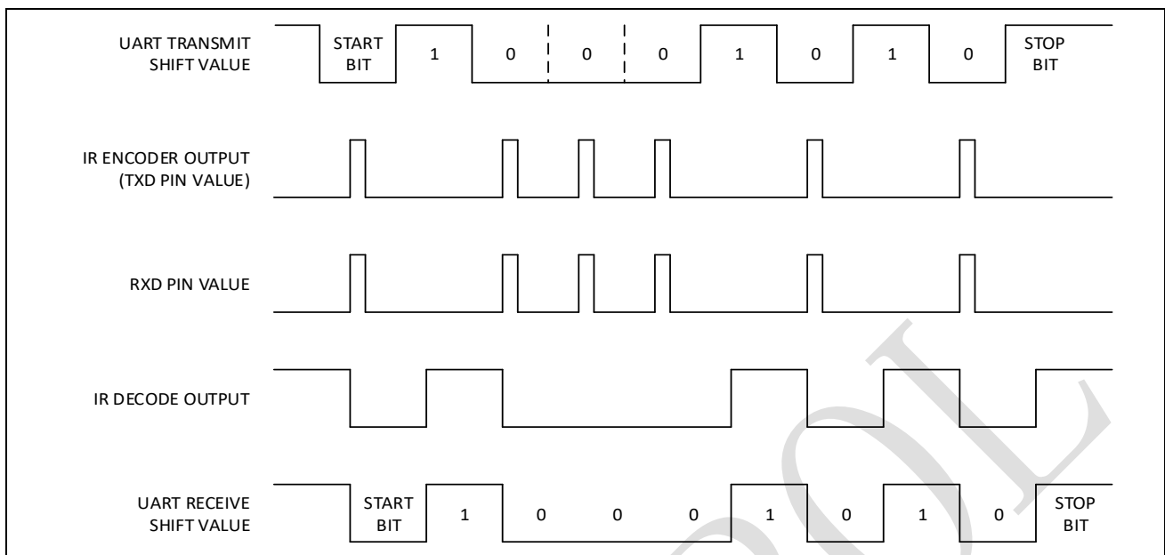
Figure 17-4: IR transmit and receive example
