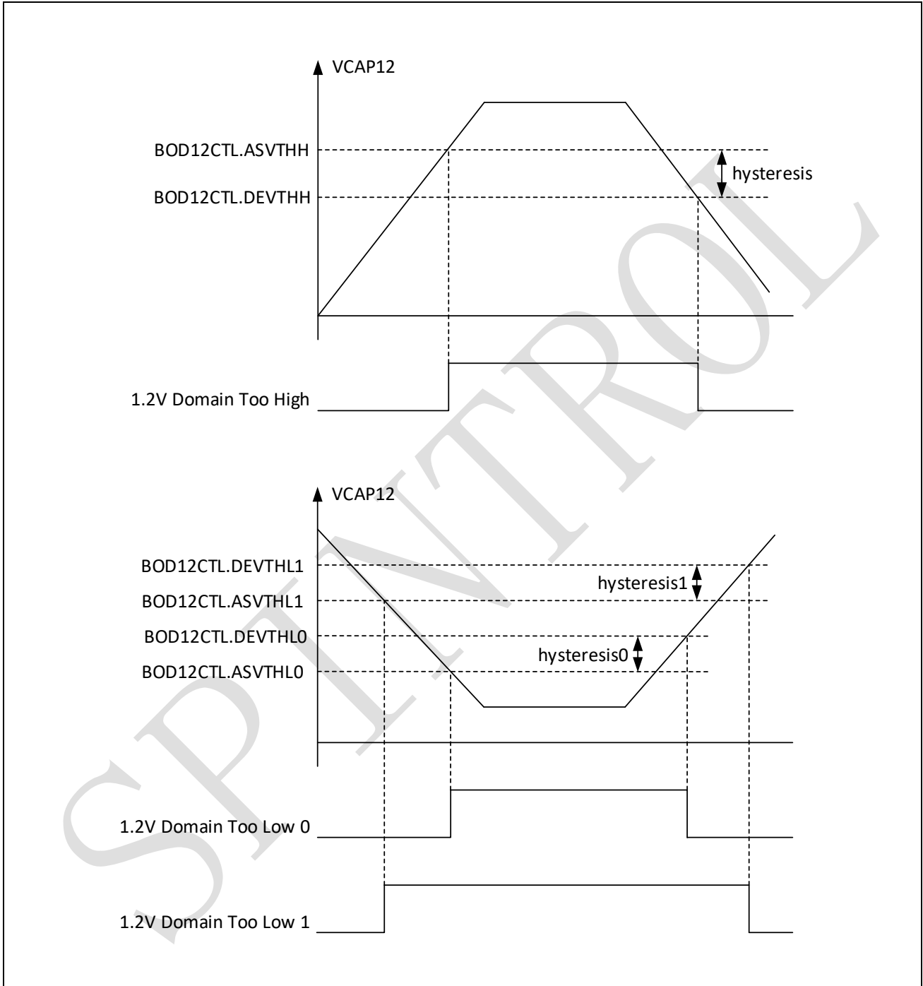
Figure 2-6: VCAP12 thresholds
