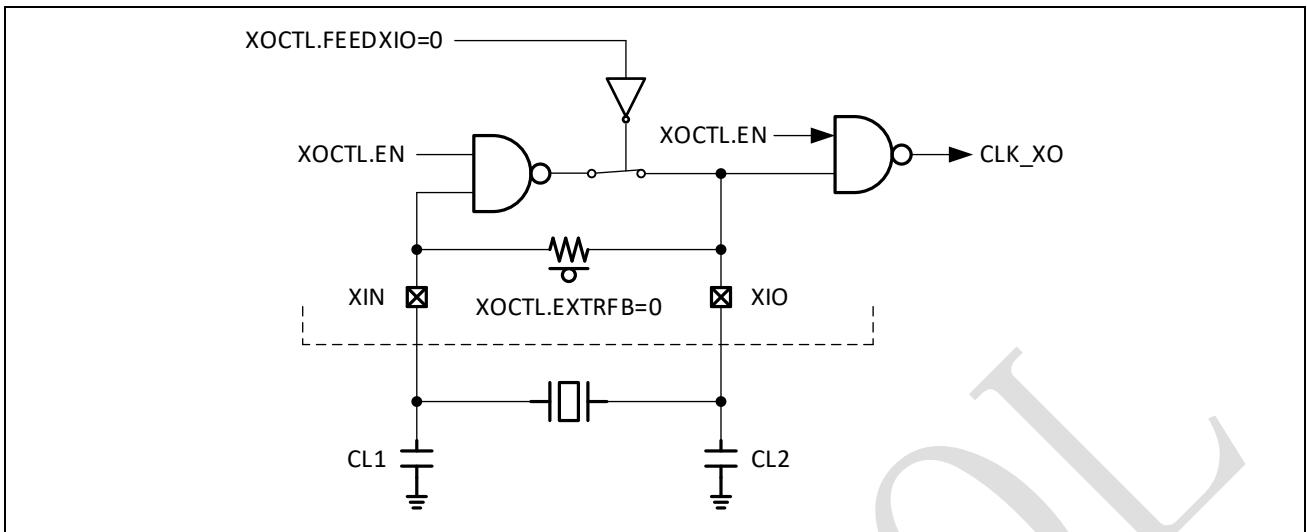
Figure 3-4: On-chip crystal oscillator
