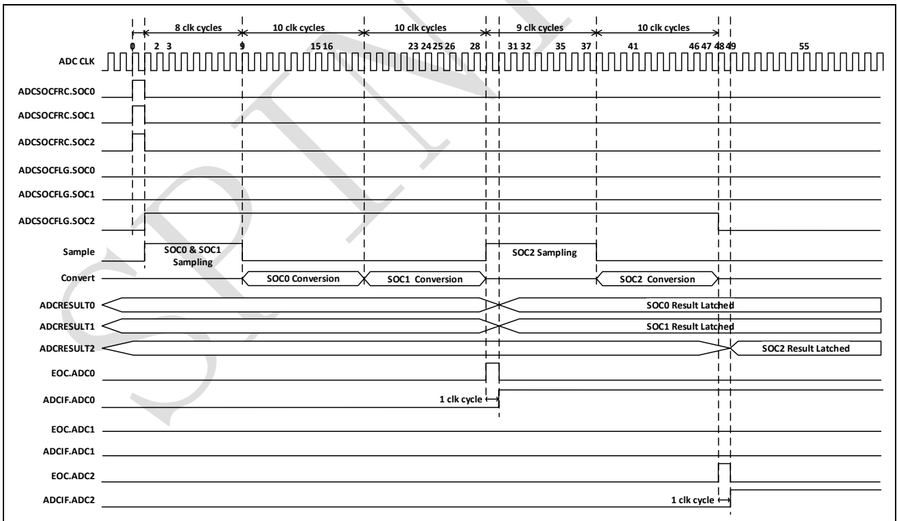
Figure 12-13: Timing example for simultaneous mode interrupt
