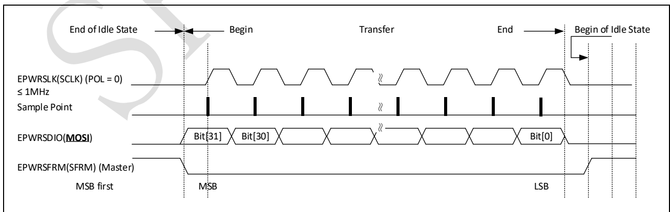
Figure 24-3: MCU Transmit Data to Pre-Driver module (PHA=0)
