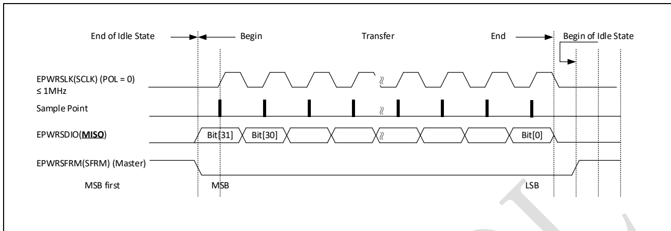
Figure 24-4: MCU Receive Data from Pre-Driver module (PHA=0)
