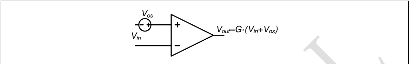
Figure 14-7: PGA offset
