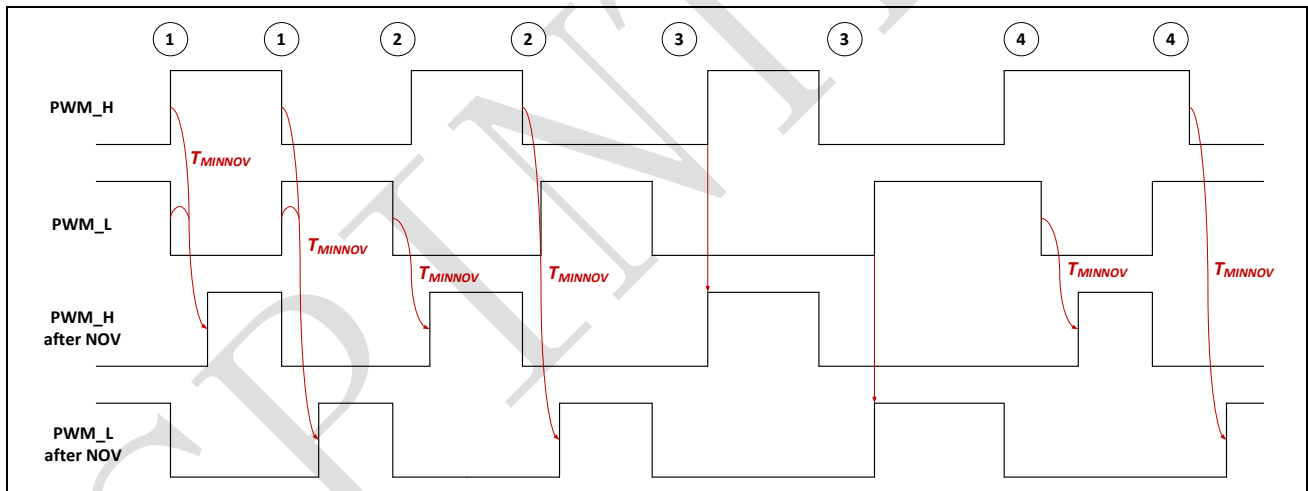
Figure 24-7: Illustration of NOV block operation
