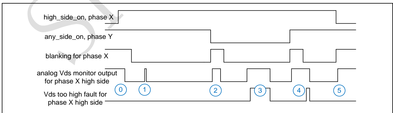
Figure 24-9: Blanking diagram of V_{ds} monitors
