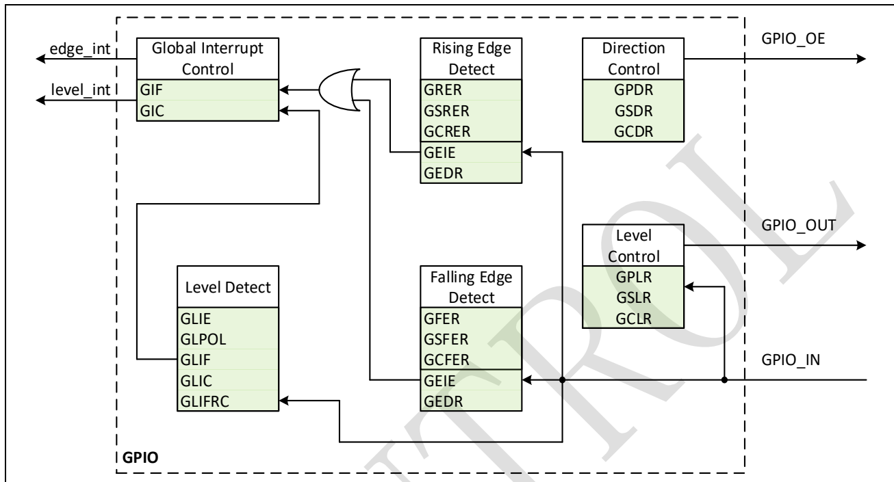
Figure 4-5: GPIO structure diagram
