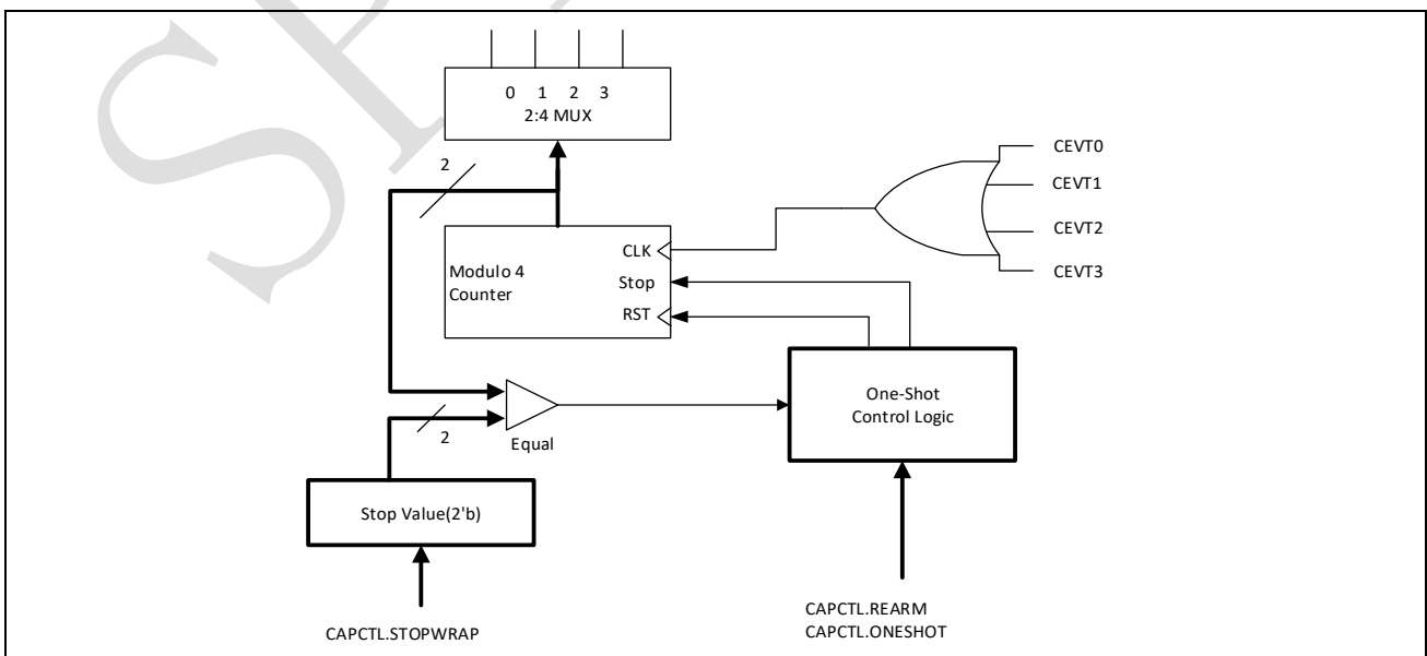
Figure 11-6: Details of the continuous/one-shot block
