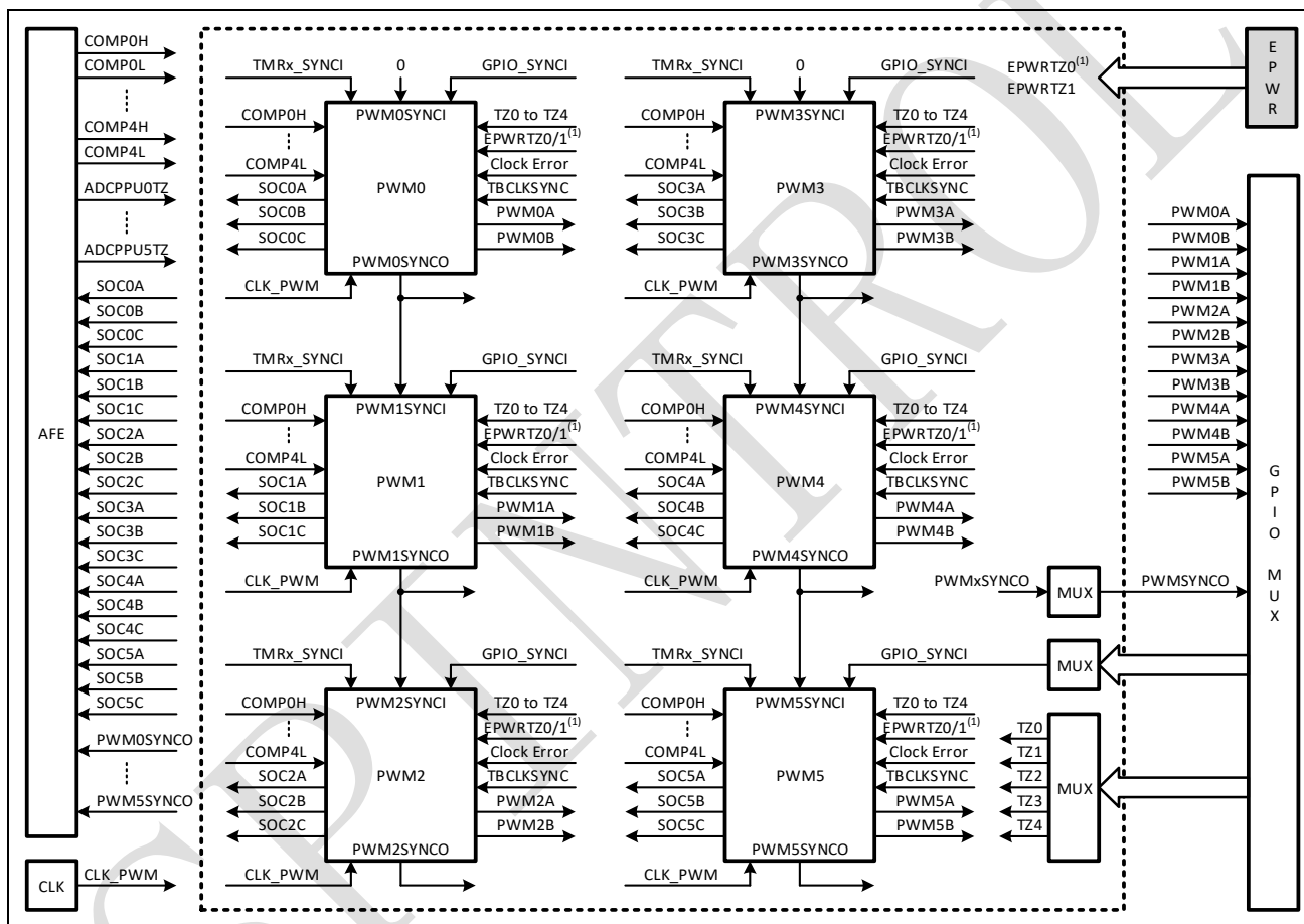
Figure 10-1: PWM overview
