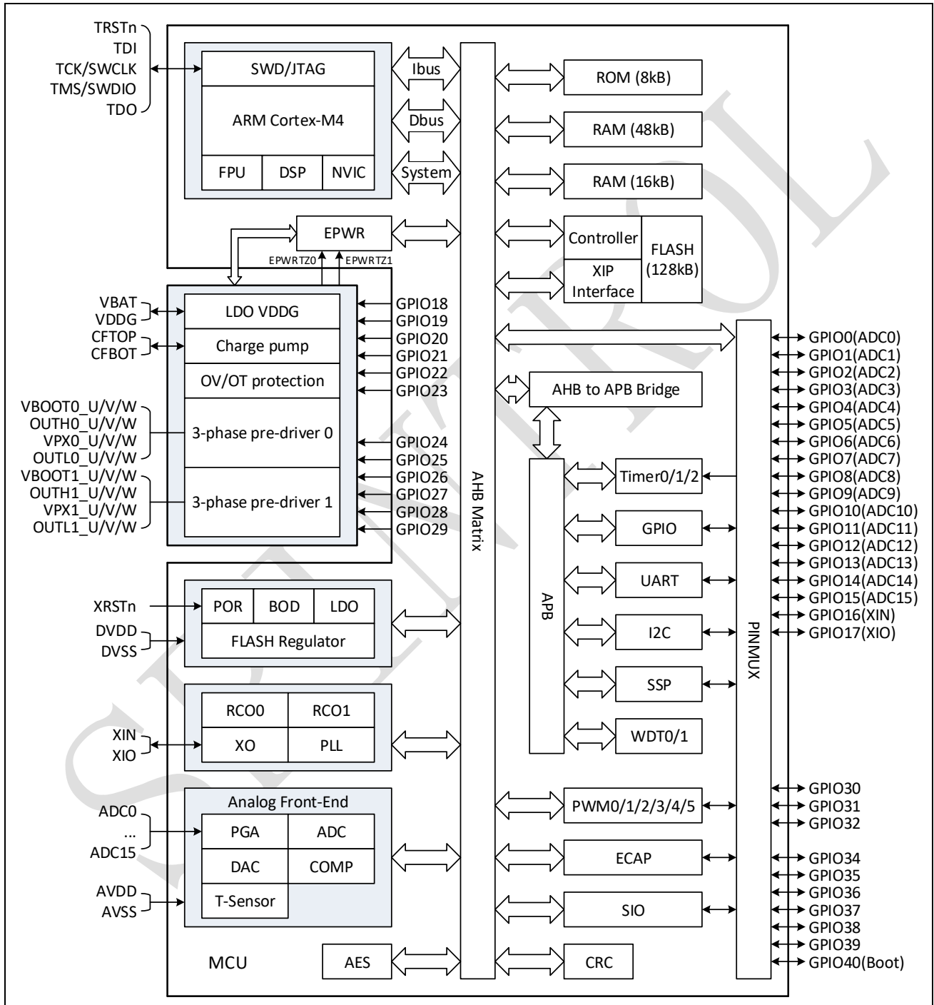
Figure 1-1: Block diagram of SPD1178
