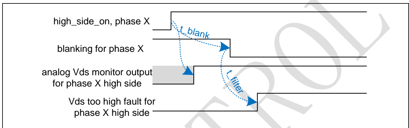
Figure 24-10: Effects of blanking and filtering on fault assertion
