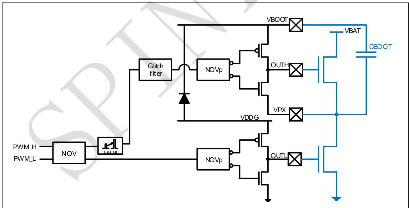
Figure 24-6: Simplified diagram of a phase of the Pre-Driver
