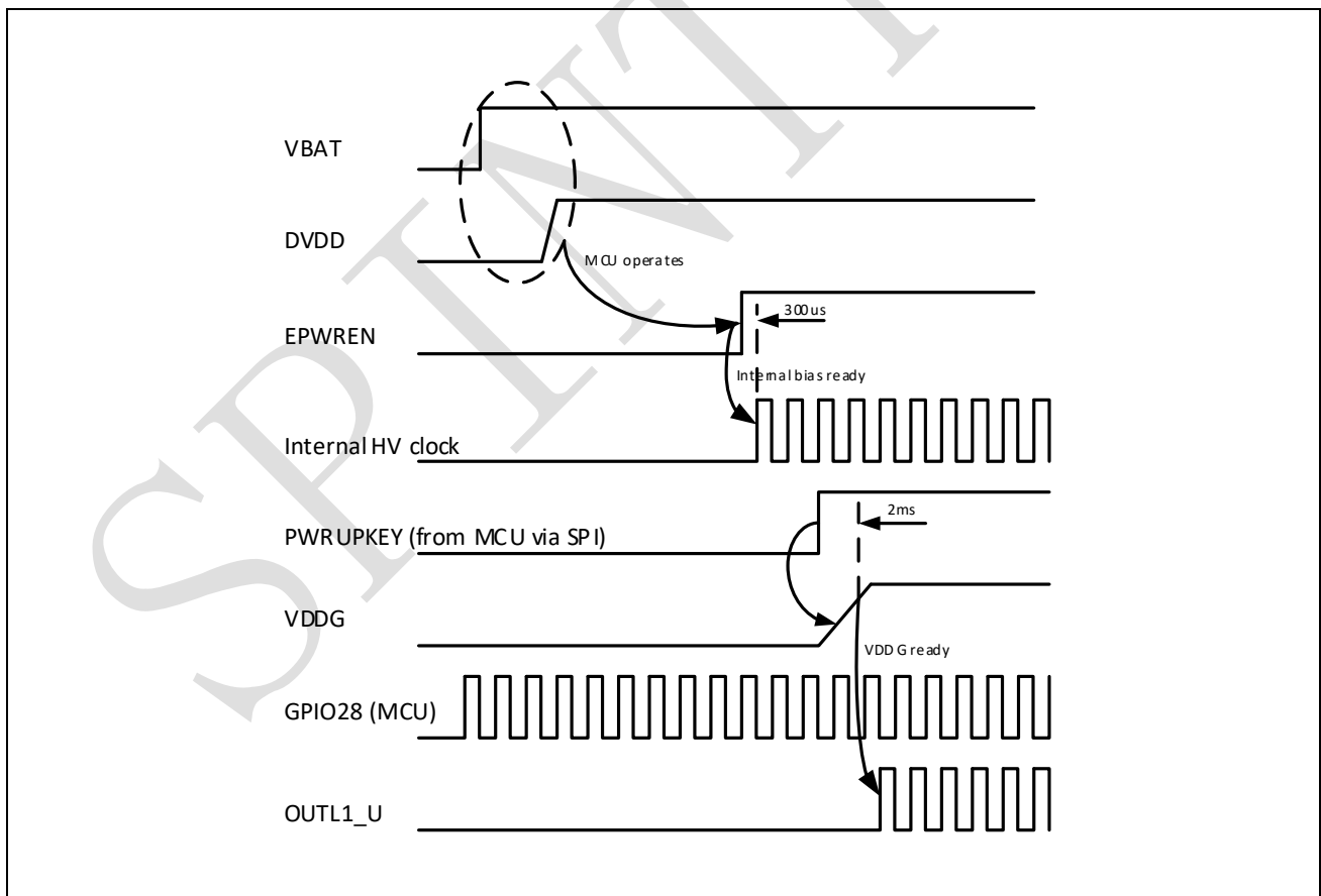
Figure 24-5: Pre-Driver signal power-up scheme
