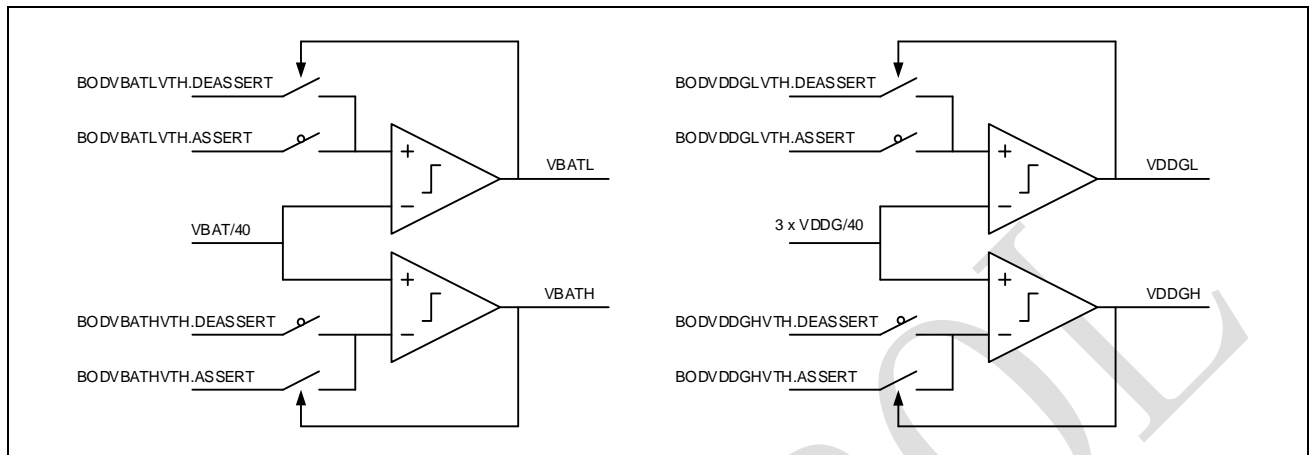
Figure 24-8: Power rail detector for VBAT and VDDG
