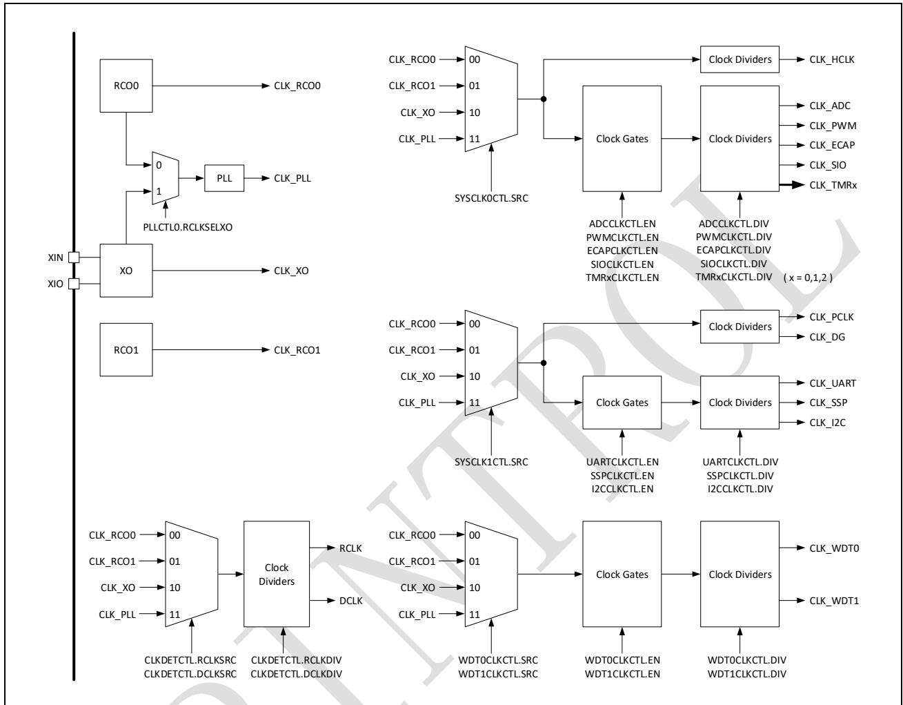
Figure 1-2: SPD1178 clock tree
