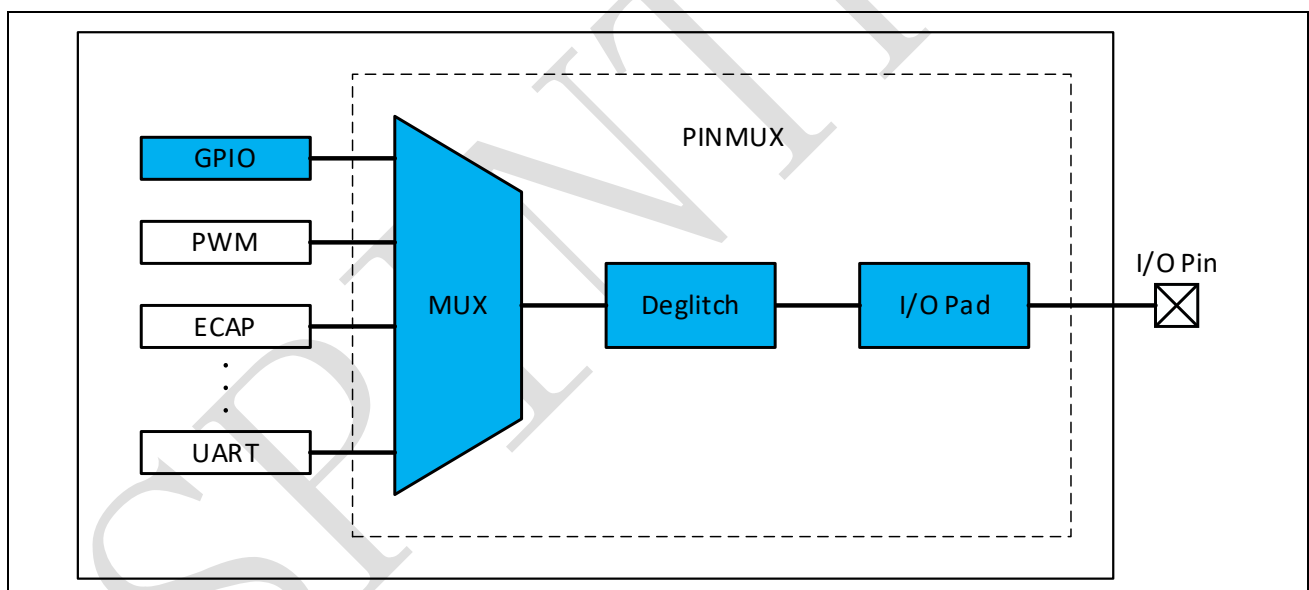
Figure 4-1: Structure diagram of I/O control
