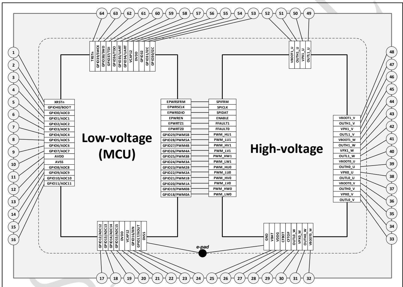
Figure 24-2: MCU and Pre-Driver module connection diagram
