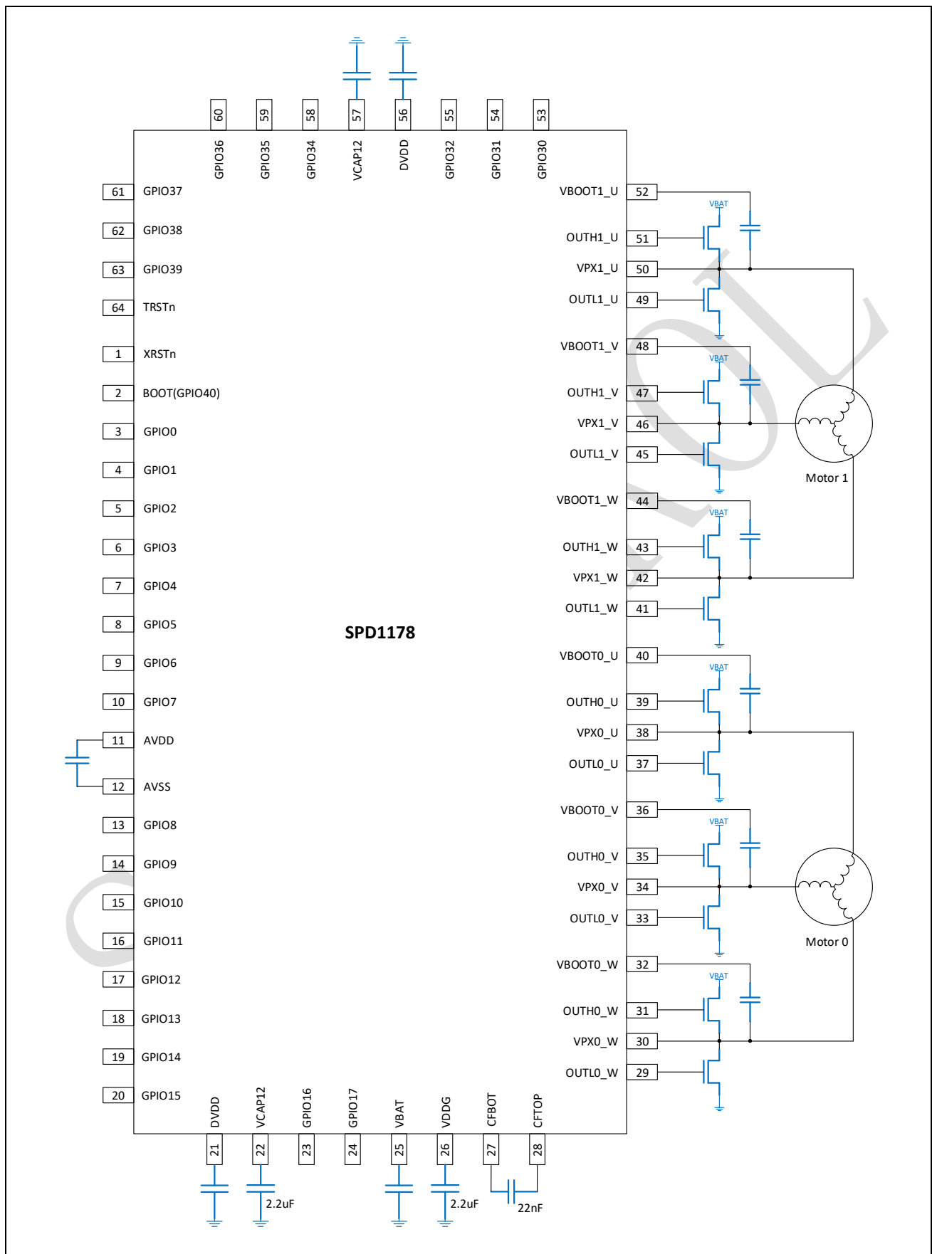
Figure 24-1: SPD1178 typical application diagram
