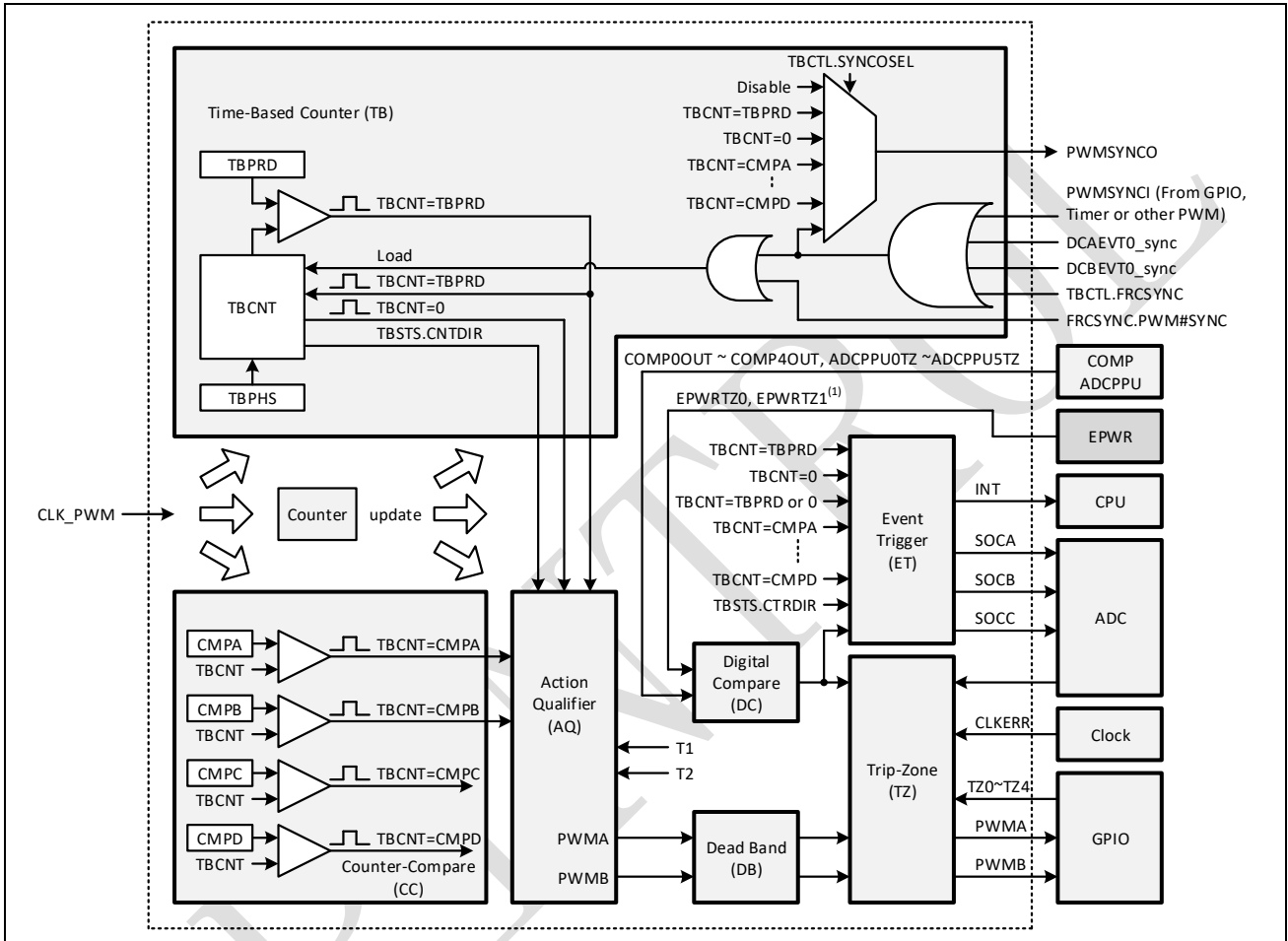
Figure 10-2: PWM architecture
