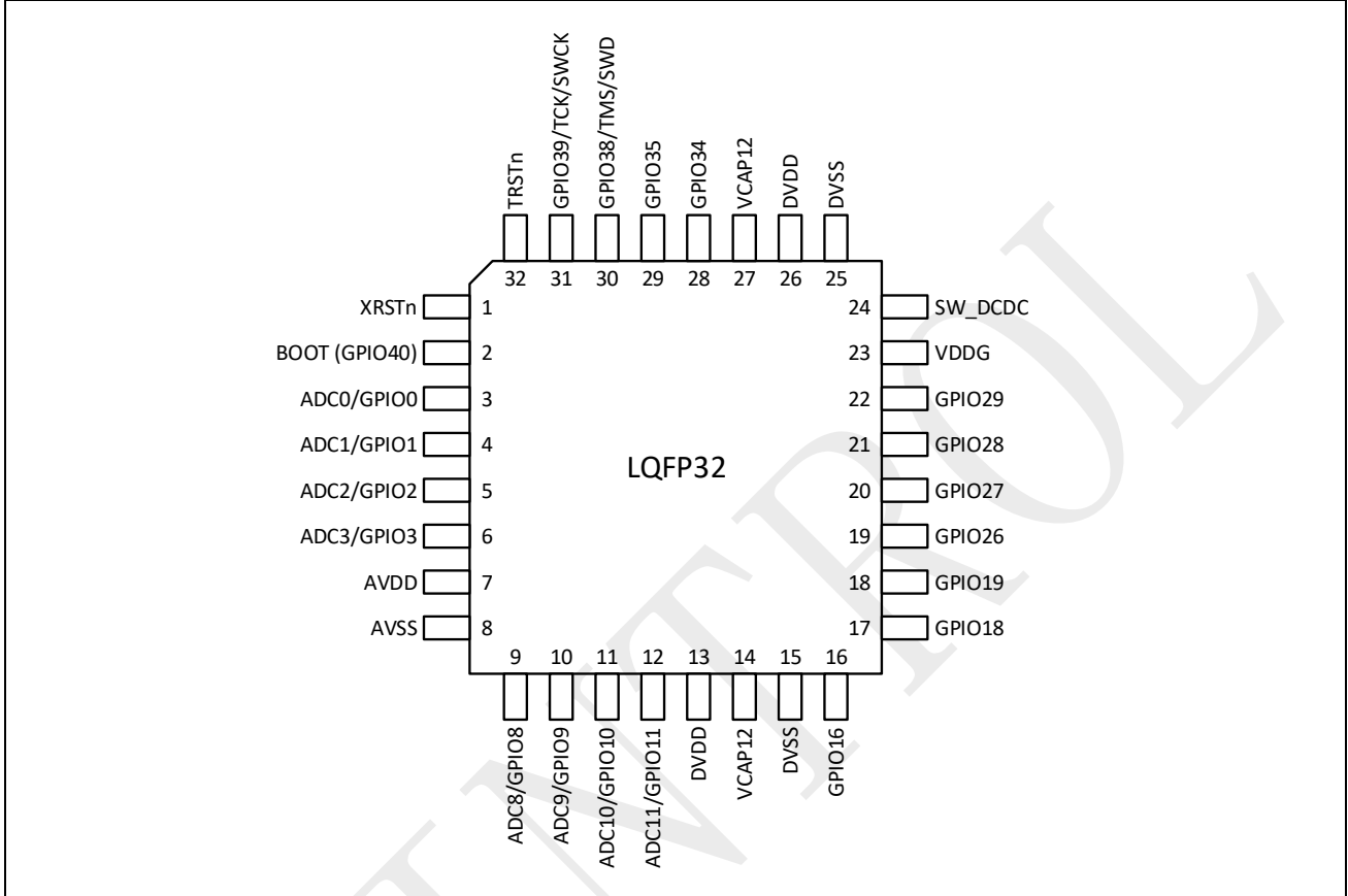
图 3-3: SPC1158 LQFP32 引脚排列
